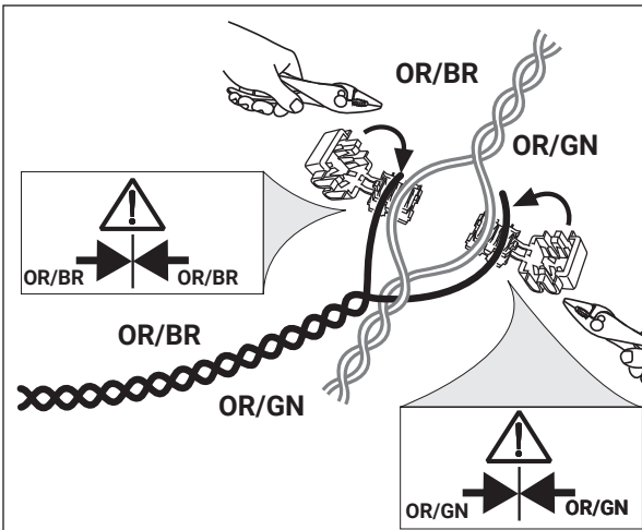
Body Control Module connector A
